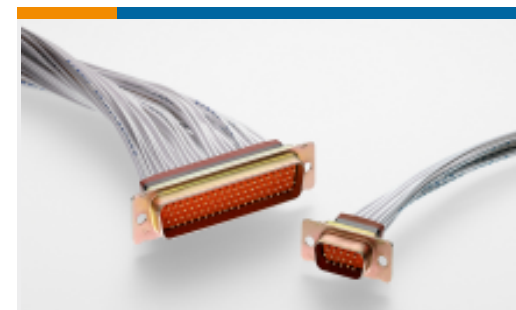
TE Part # 1-2221860-2 AMPLIMITE IP67,SZ2, 90, 26 POS,IFS, PLUG
